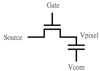
Figure 7-8 : Vpixel Definition
